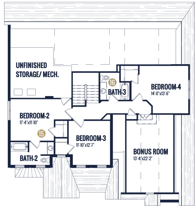
UPPER LEVEL
