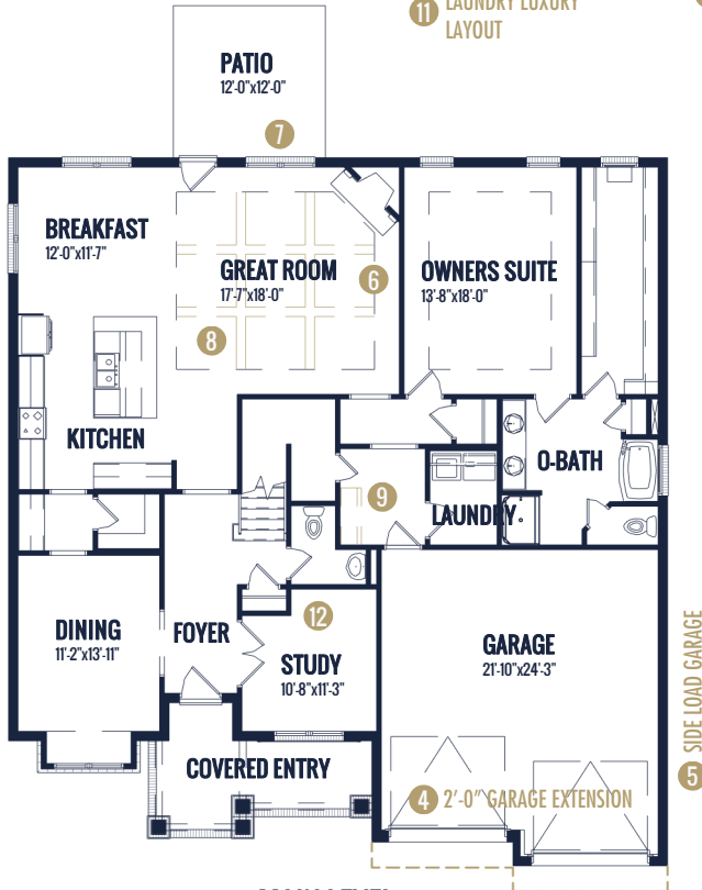
MAIN LEVEL
